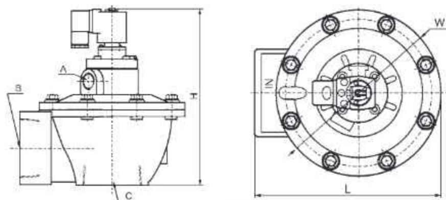
DMF-Z-40S/50S/62S/76S
