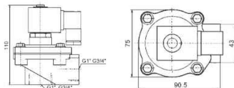
DMF-Z-40S/50S/62S/76S
